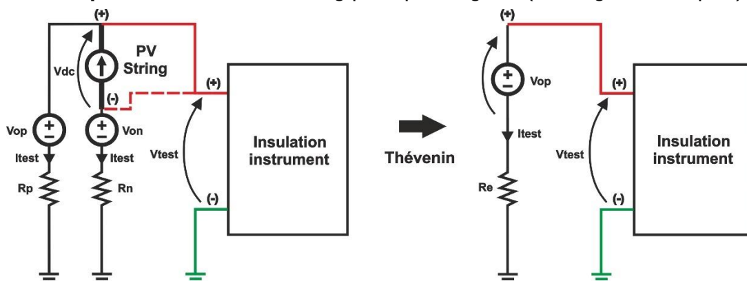
Fig. 15: Diagram and equivalent circuit of Method 1
